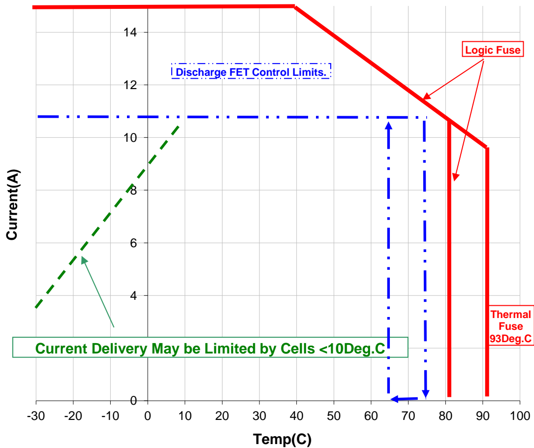
Discharge Operating Limits
