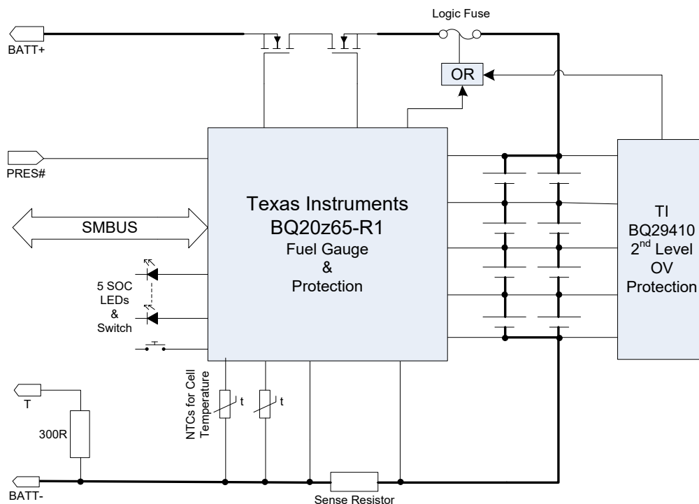
Figure 2 - Battery Pack Electronics Block Diagram
