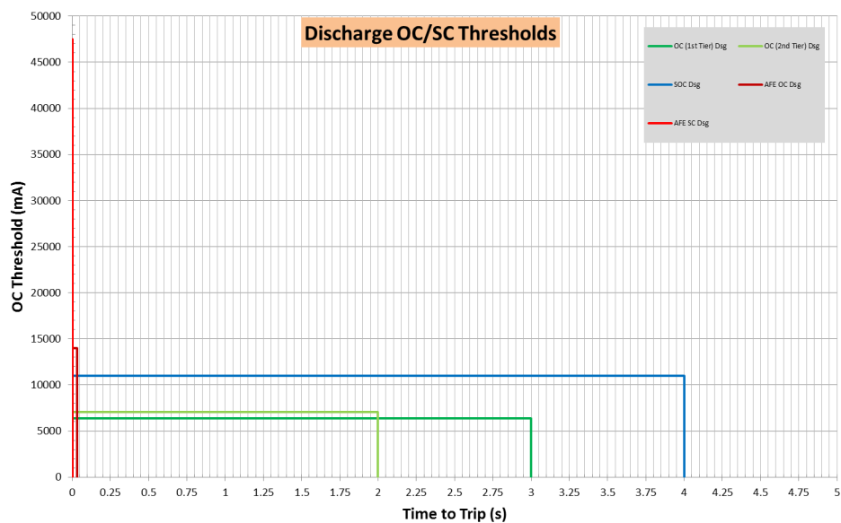
Figure 4 - Discharge OC/SC Protection Values
