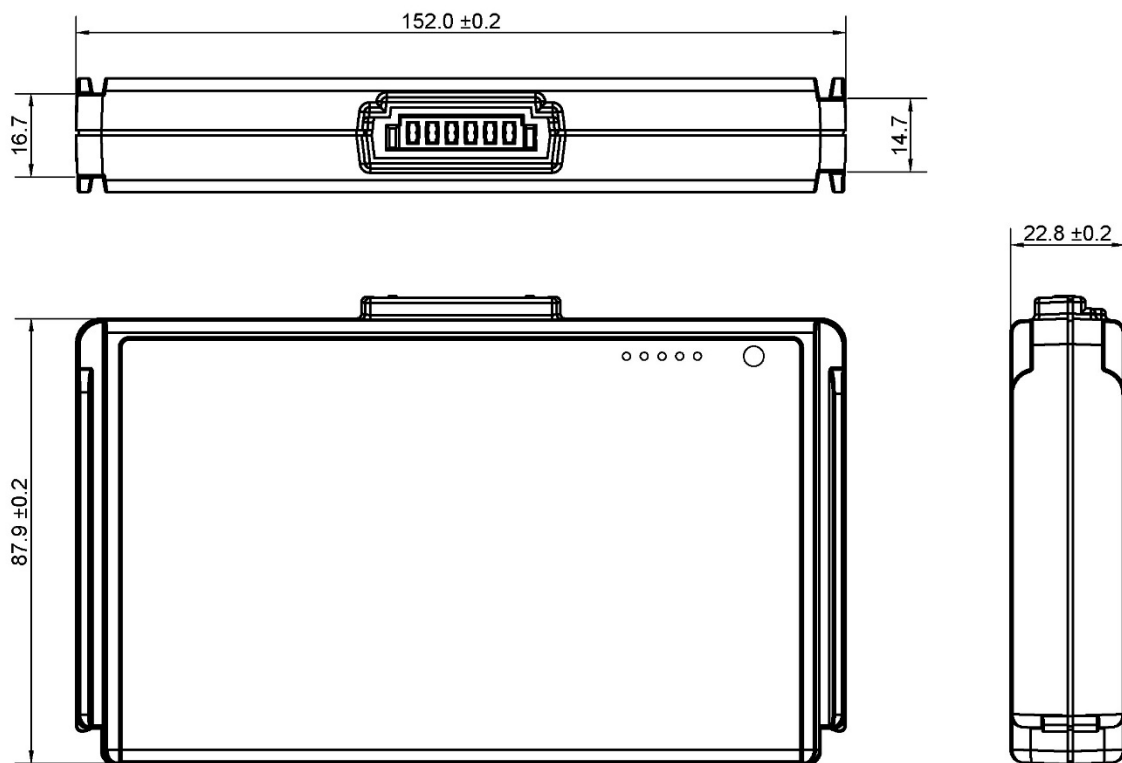
Figure 5 - Mechanical Drawing
