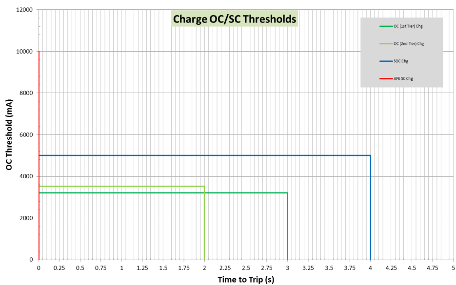
Figure 3 - Charge OC/SC Thresholds
